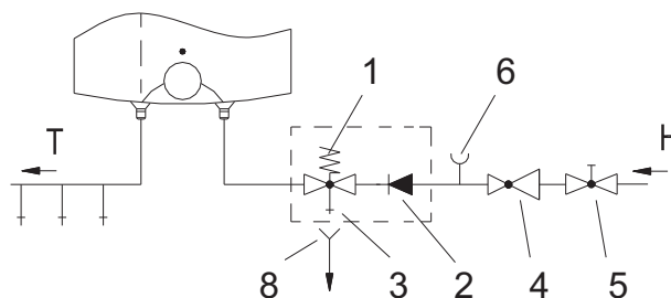
Installation above the basin/sink
