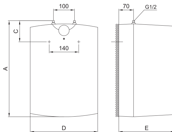
Installation below the basin/sink
