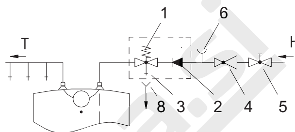
Installation below the basin/sink
