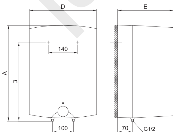
Model nad umivaonikom
