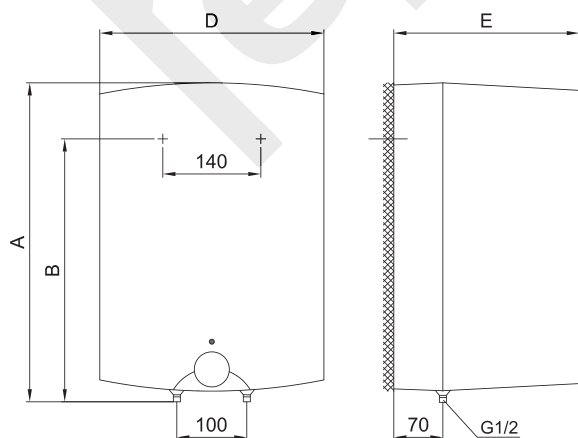
Installation above the basin/sink
