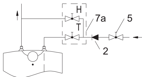
Installation below the basin/sink
