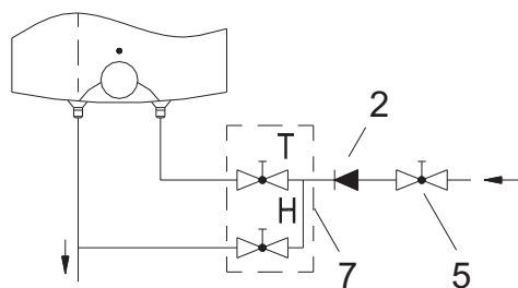
Installation above the basin/sink
