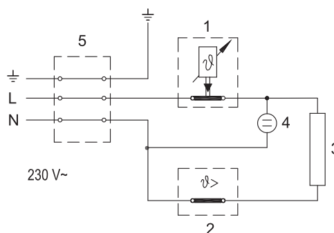
Electric installation
